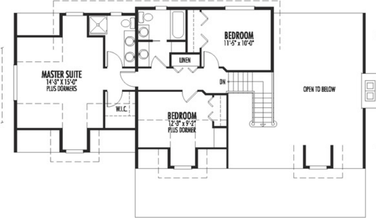
Upper Floor 883 sq.ft.
